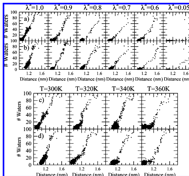
Figure 4. Number of interpeptide water molecules is plotted against the interpeptide distance for the two trajectories in which a drying transition was not observed using the original potential function. In each simulation the initial conditions are the same as those in Figure 3a and b, D_0 is 1.28 nm, and the temperature is 300 K. (a and b) The van der Waals attraction between the peptide and water has been scaled by a factor of \lambda^a (such that \lambda^a = 1 is the full potential used in Figure 3a,b). In each case the repulsive term of the van der Waals interaction is unchanged. (c and d) Each simulation is performed at a different temperature.
